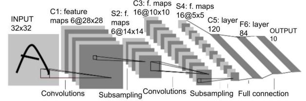
Figure 1. Architecture of the LeNet5 CNN [17].
